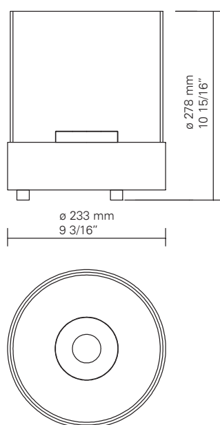
Technical drawing
